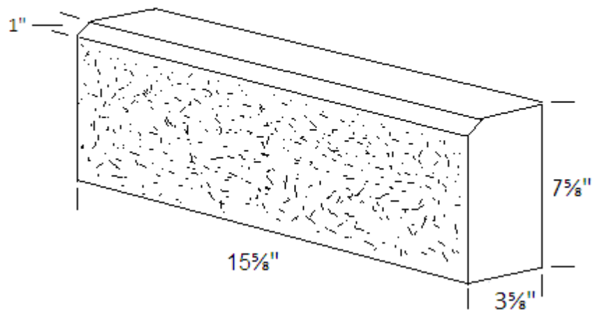
4"x8"x16" SPLITFACE SILL w/ \frac{3}{4} "x \frac{3}{4} " CHAMFER
