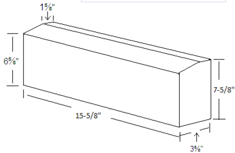
4x8x16 SOLID SILL w/ 2" x 1" CHAMFER
