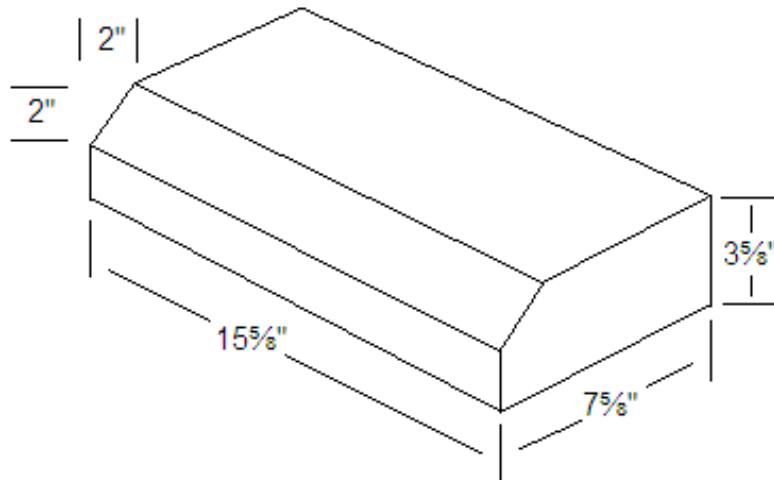
8x4x16 Solid Sill with \frac{3}{4} " x \frac{3}{4} " Chamfer
