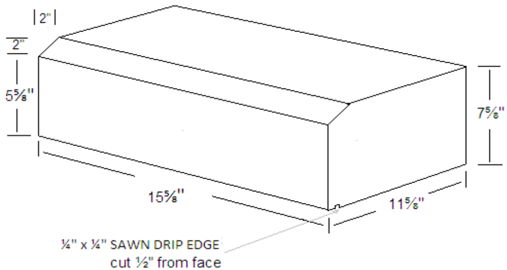
12x8x16 SILL with 2" x 2" CHAMFER
