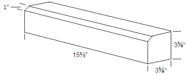
4x4x16 SILL UNIT - \frac{3}{4} " x \frac{3}{4} " CHAMFER
