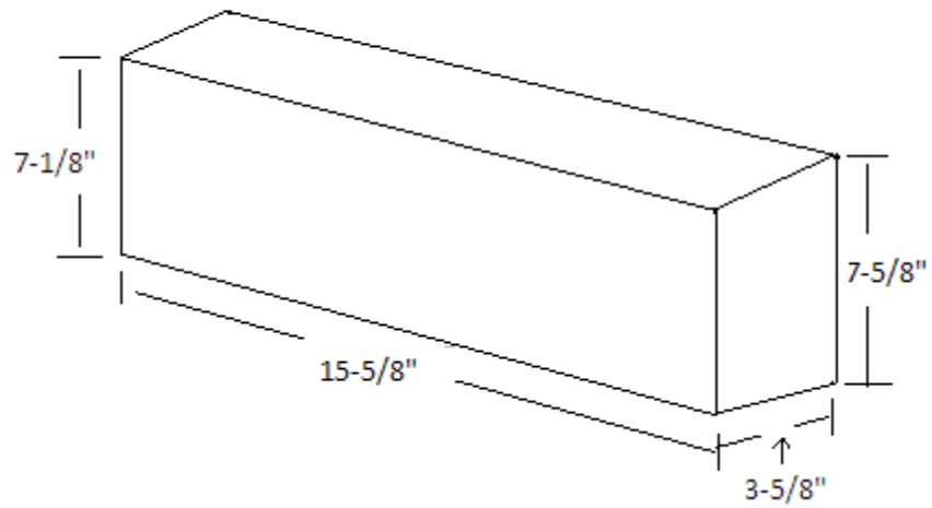
4x8x16 SLOPED SILL UNIT
