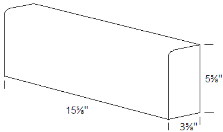
4 x 6 x 16 Bullnose Sill Unit
