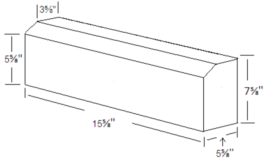
6x8x16 SILL with 2" x 2" CHAMFER
