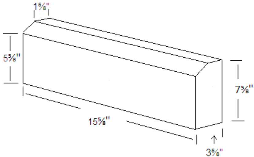
4x8x16 SILL w/ 2"x2" CHAMFER
