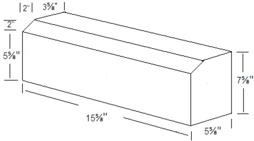
6x8x16 SILL with 2" x 2" CHAMFER
