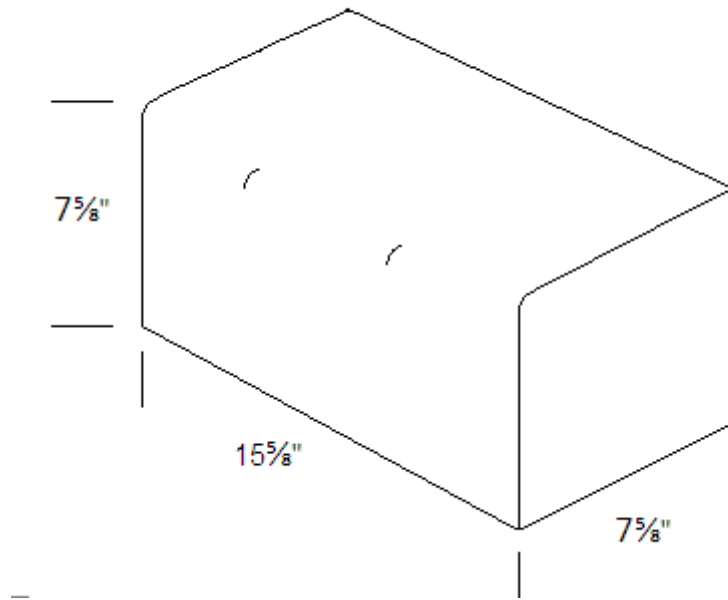
8x8x16 Solid Sill - 1Face, 1Top, 1BN Top Edge, 1 End
