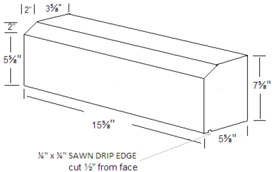
6x8x16 SILL with 2" x 2" CHAMFER
