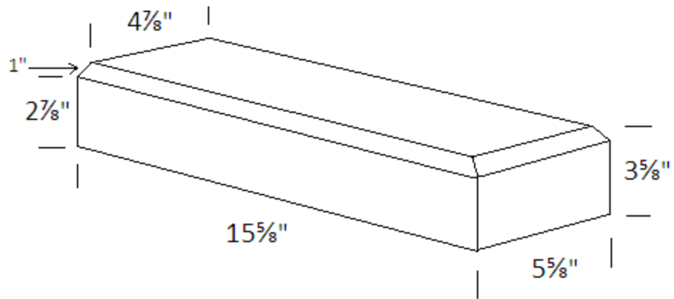
6x4x16 Sill Unit - \frac{3}{4} " x \frac{3}{4} " Chamfer and Chamfer Return
