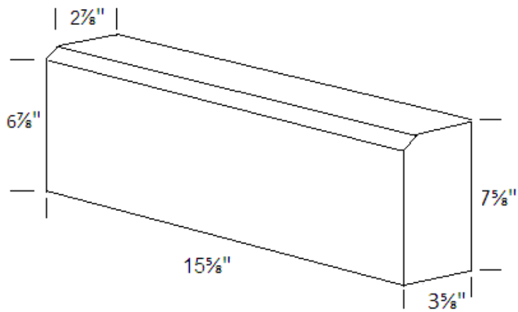
4"X8"X16" SILL w/ \frac{3}{4}" X \frac{3}{4}" CHAMFER
